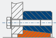
Model AB: Thread in the outer ring and centring device
