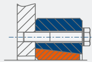
Model C: Thread in the attachment
